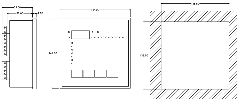
CRK L8 / 12D
