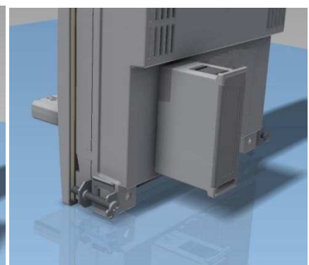
Expansion mounting
